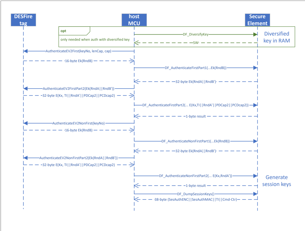
Figure 19. Example DESFire authentication using SE05x
