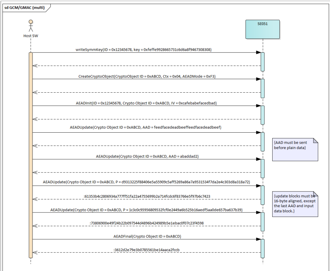
Figure 24. Example GCM operation in multiple steps (P2_ENCRYPT)
