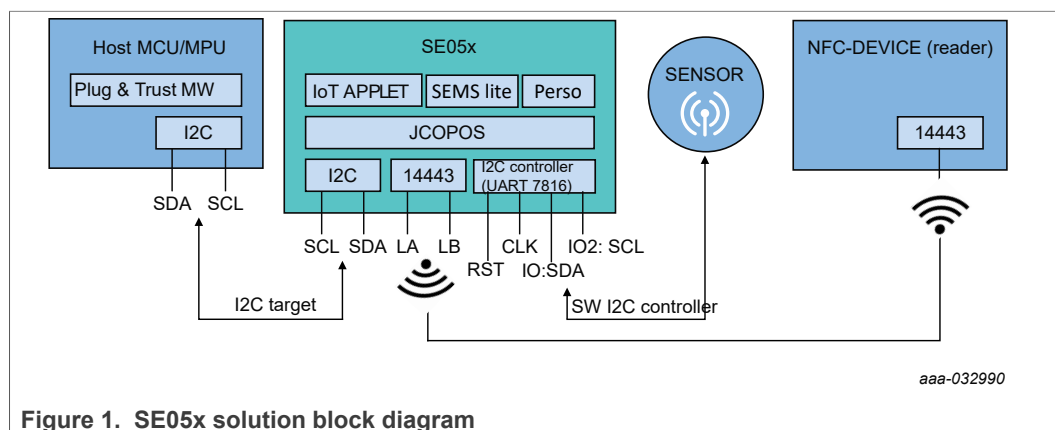
Figure 1. SE05x solution block diagram
