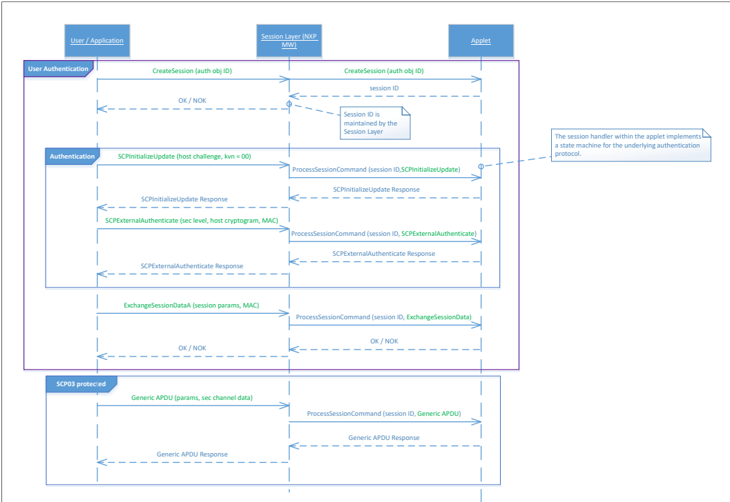
Figure 12. Session creation using an AES key as authentication object
