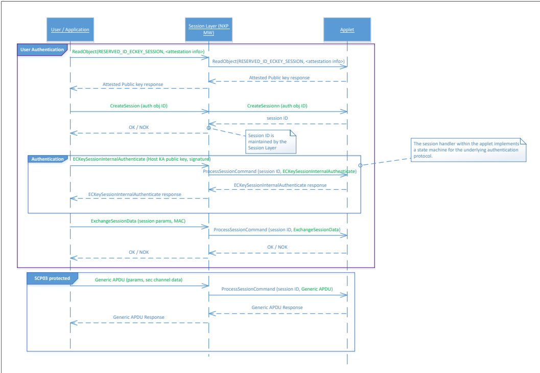
Figure 13. Session creation using ECKey session as authentication mechanism.
