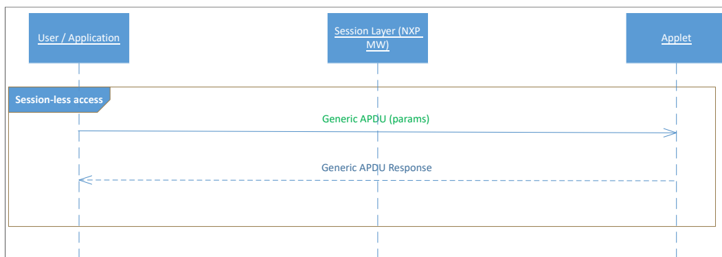
Figure 9. Session-less access
